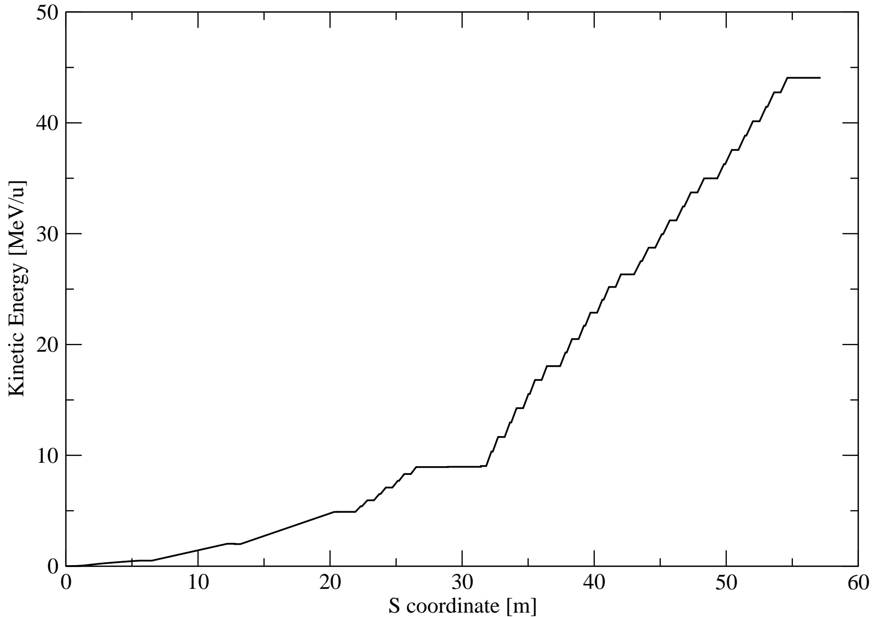
JLEIC Ion Linac (Pb, low energy option)
