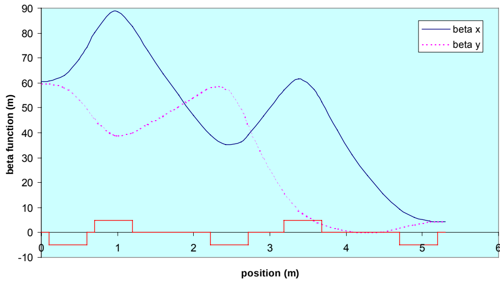
Fig. 3.1.5-3. Matching of the \beta -functions from the linac to the TBA cell.
