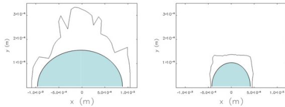
Figure 2: Dynamic apertures with multipole fields of the arc dipoles (left: errors in arc dipoles with \beta < 200 m; right: errors in all arc dipoles).
