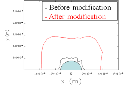
Figure 6: Dynamic apertures with the multipole fields of the IR triplets (black: original data; red: modified data).
