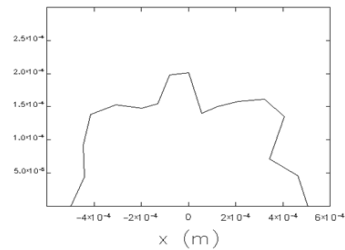
Figure 3: Dynamic aperture of the JLEIC ion ring where the LHC triplets multipole field is applied to the JLEIC triplets.
