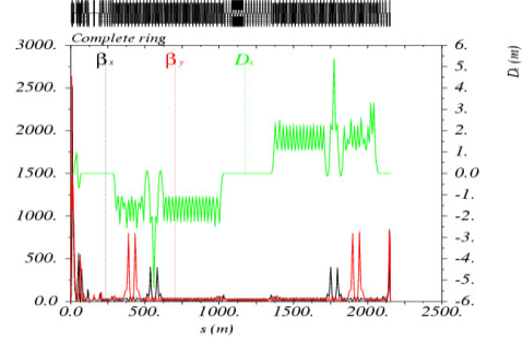
Figure 1: Linear optics of the JLEIC ion collider ring starting from IP.
