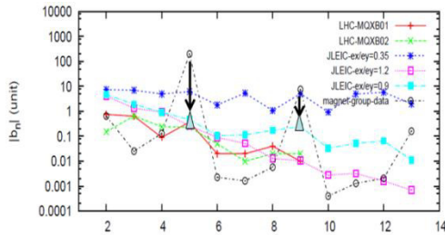
Figure 5: Preliminary multipole field data (black dash) and the modification of b5 and b9 (arrow and triangle).
