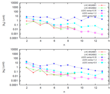
Figure 4: Survey of limiting multipole field coefficients in the JLEIC ion collider ring.
